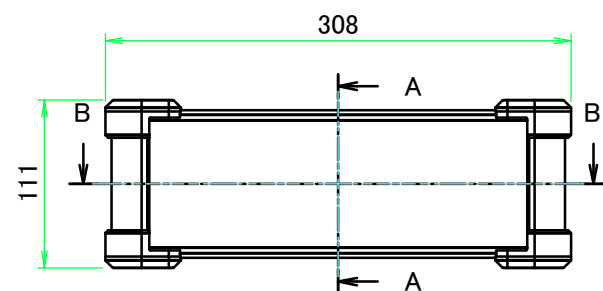
A view
