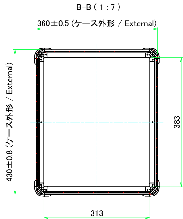
D view
