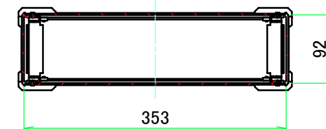
C-C (1:7)
