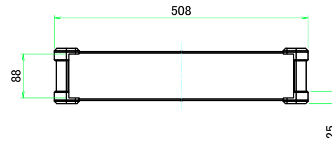
C view
