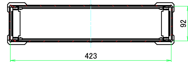
C-C (1:6)
