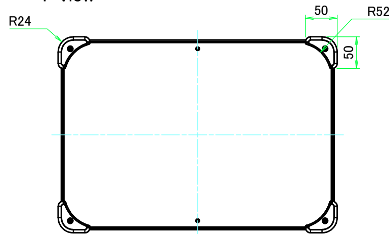
F view
