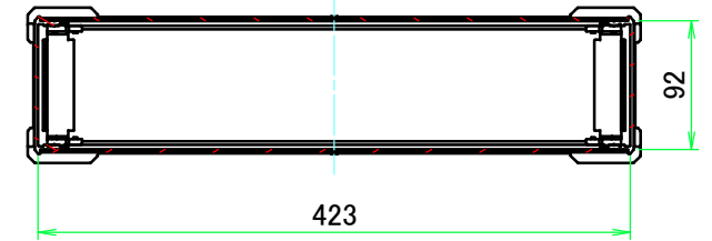
C-C (1:6)
