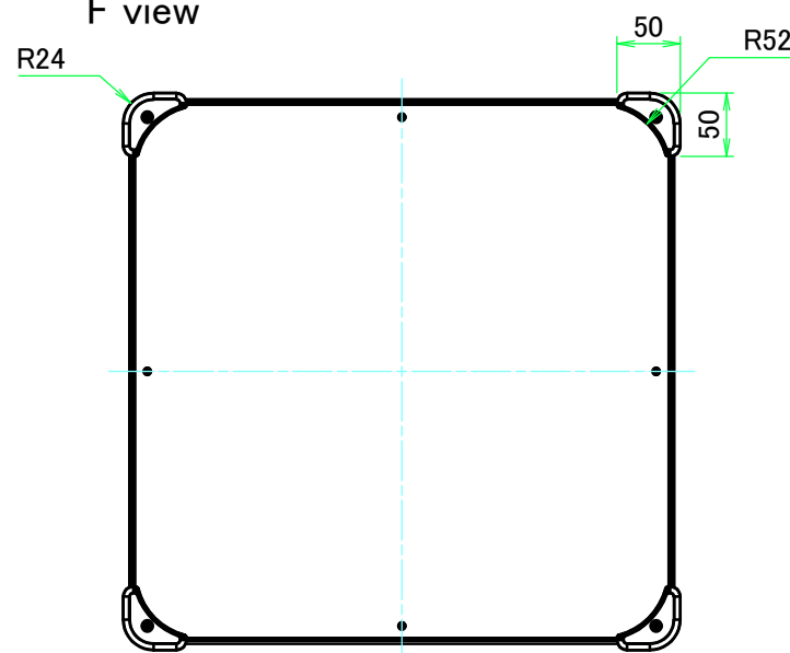
F view
