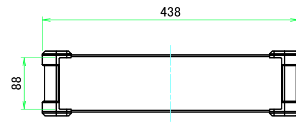
C view
