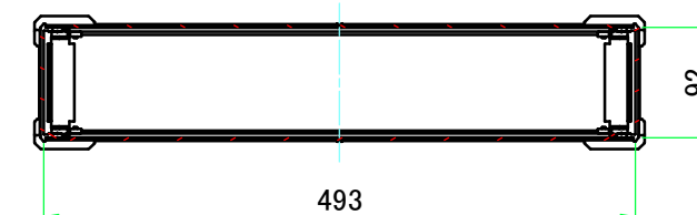
C-C (1:7)
