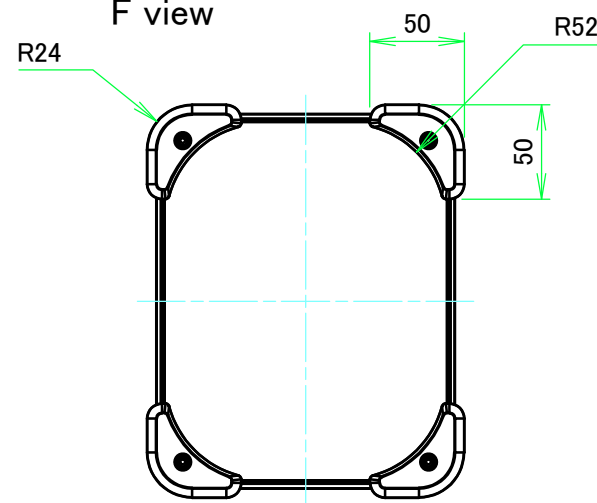
F view
