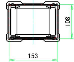
C-C (1:6)
