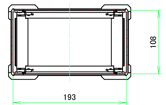
C-C (1:4)
