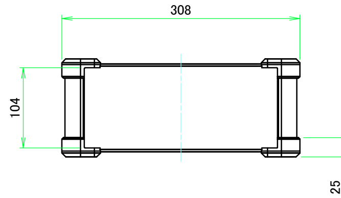
C view
