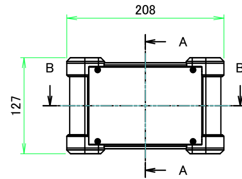
A view
