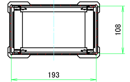
C-C (1:5)
