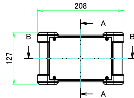
A view
