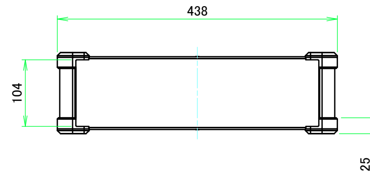
C view
