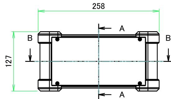
A view
