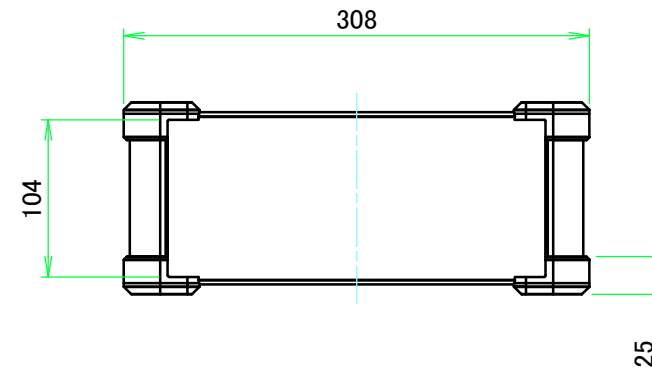
C view
