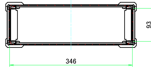
A-A (1:5.5)
