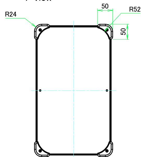
F view
