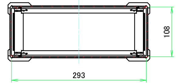
C-C (1:5)
