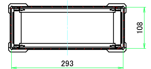
C-C (1:6)
