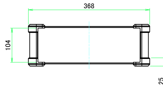
C view
