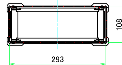
C-C (1:7)
