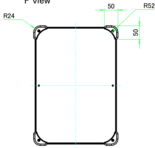
F view
