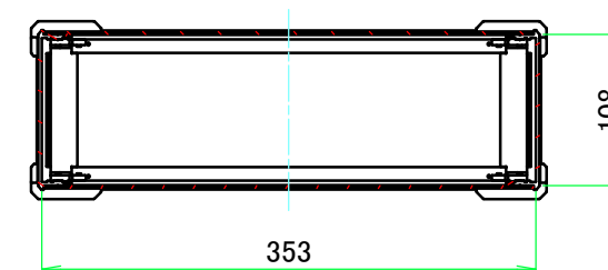
C-C (1:6)
