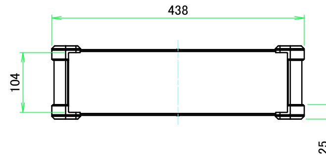
C view
