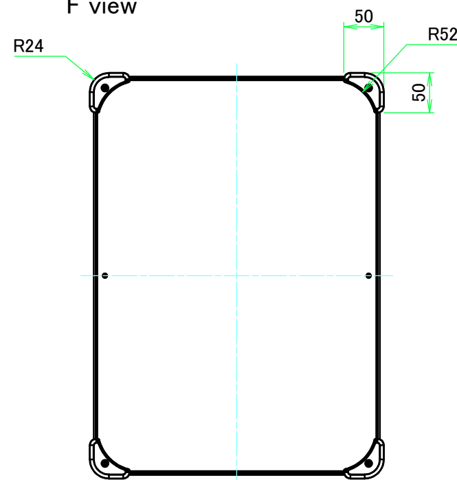
F view
