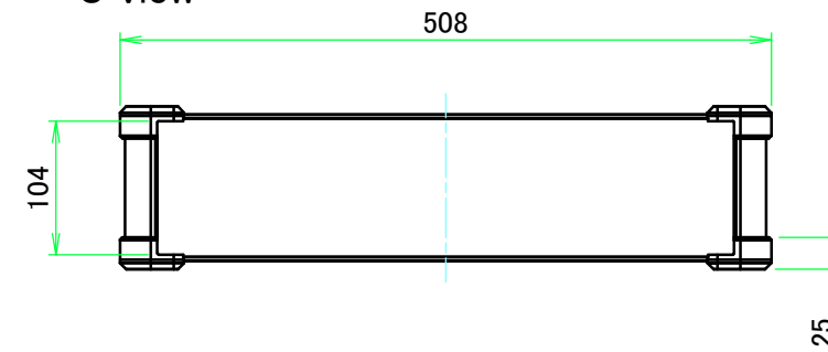
C view
