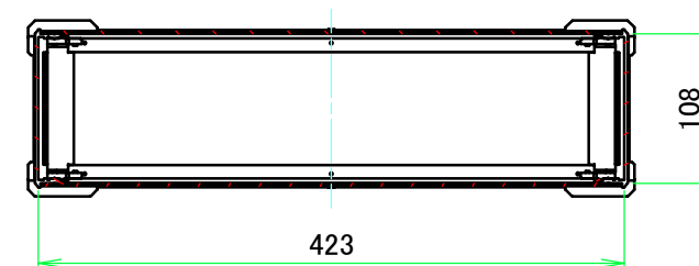
C-C (1:6)
