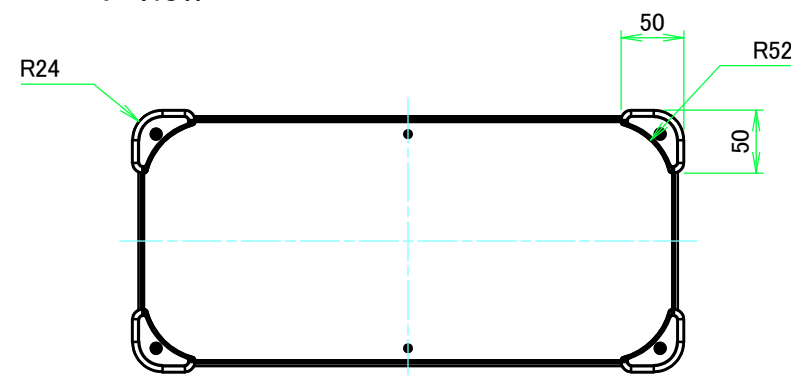
F view
