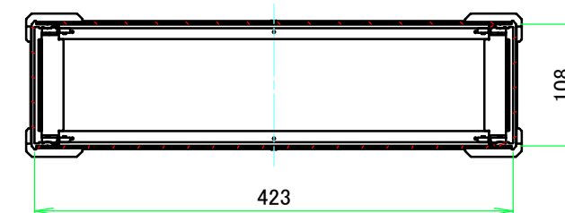
C-C (1:6)
