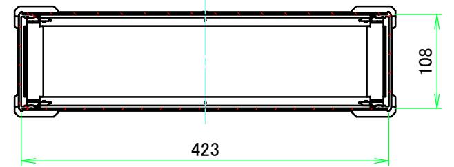
C-C (1:6)
