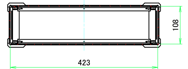
C-C (1:6.5)
