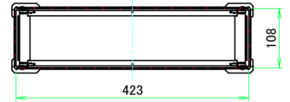
C-C (1:7)
