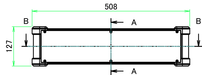
A view
