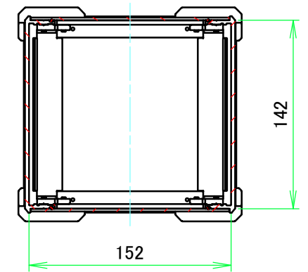
C-C (1:4)
