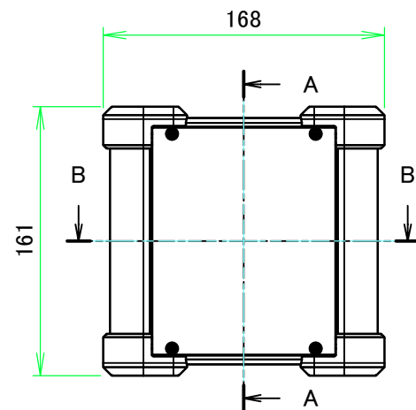
A view
