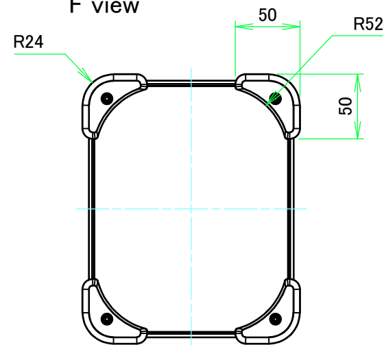
F view
