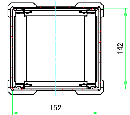
C-C (1:4)
