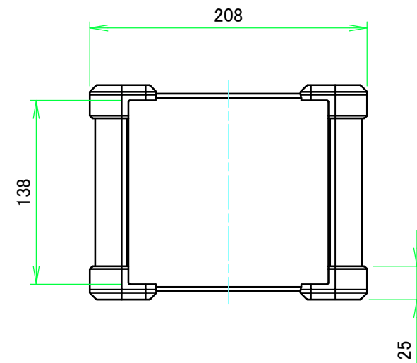
C view
