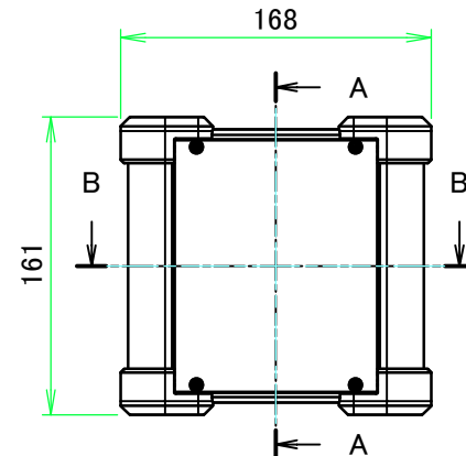
A view
