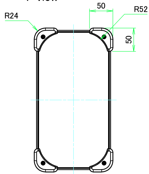
F view
