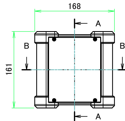
A view
