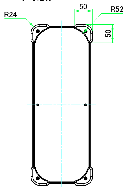
F view
