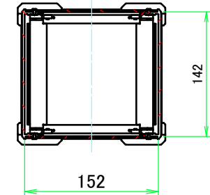
C-C (1:6)
