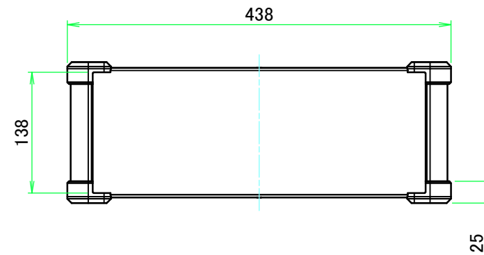
C view
