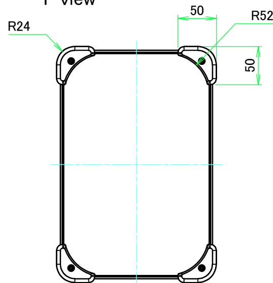
F view
