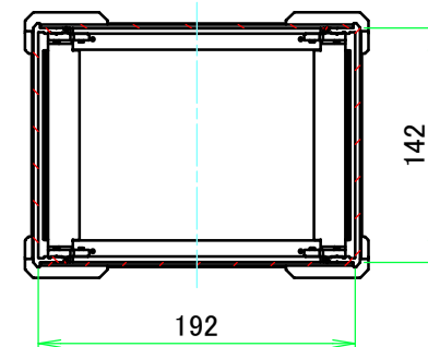
C-C (1:5)
