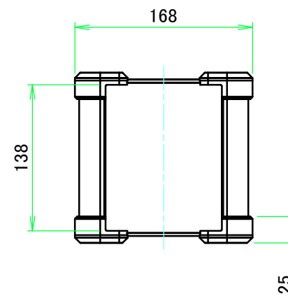
C view
