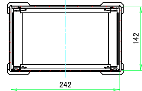
C-C (1:5)
