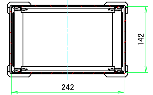
C-C (1:5)
