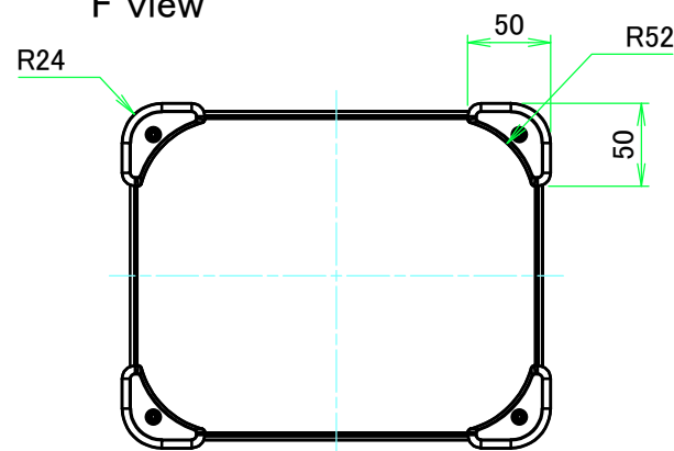
F view
