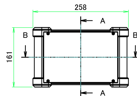
A view
