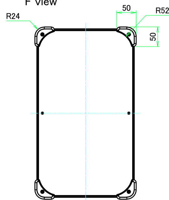
F view
