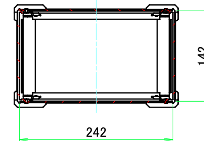
C-C (1:6)
