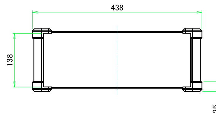
C view
