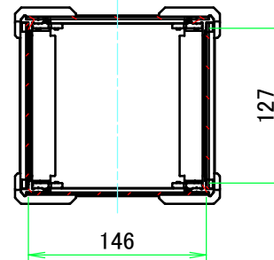
A-A (1:5.5)
