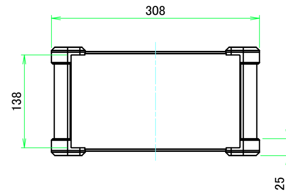
C view
