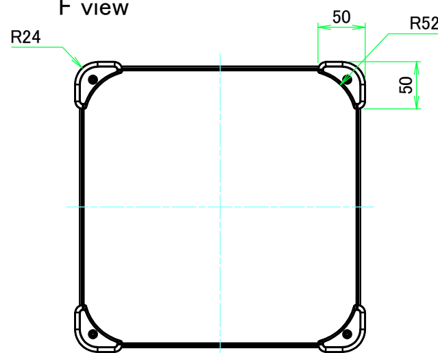
F view
