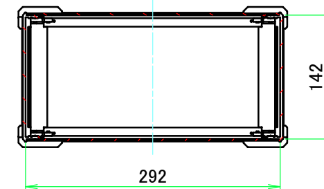
C-C (1:6)
