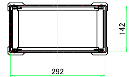
C-C (1:7)
