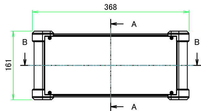
A view
