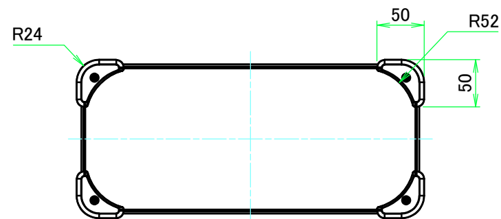
F view
