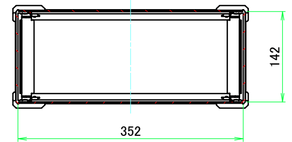
C-C (1:6)
