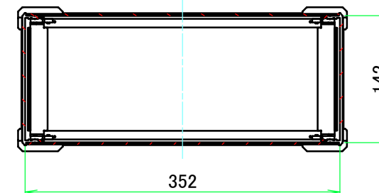
C-C (1:6)
