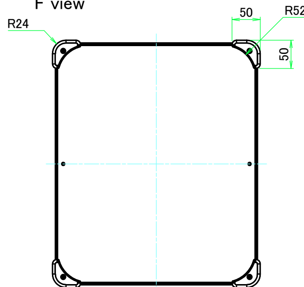
F view
