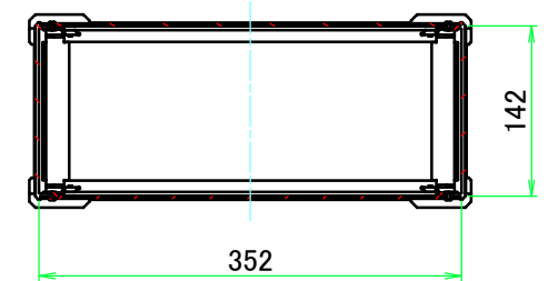
C-C (1:7)
