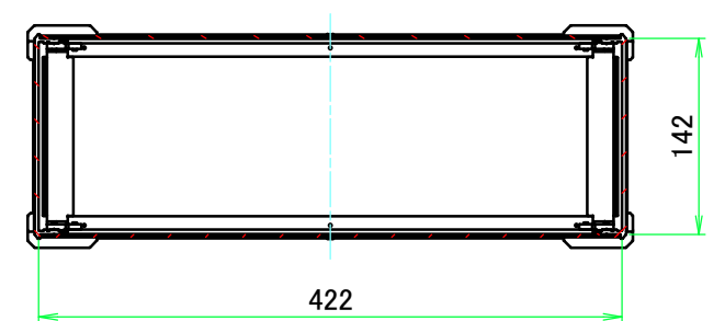
C-C (1:6)
