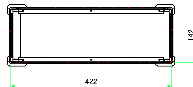
C-C (1:6)
