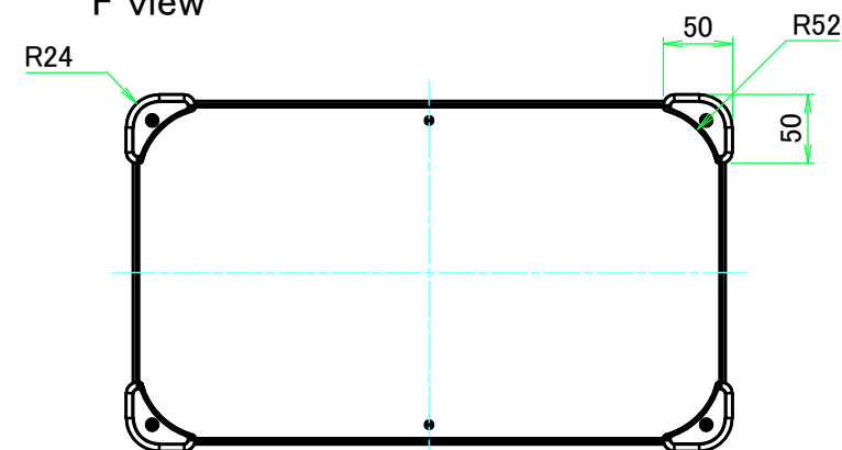
F view
