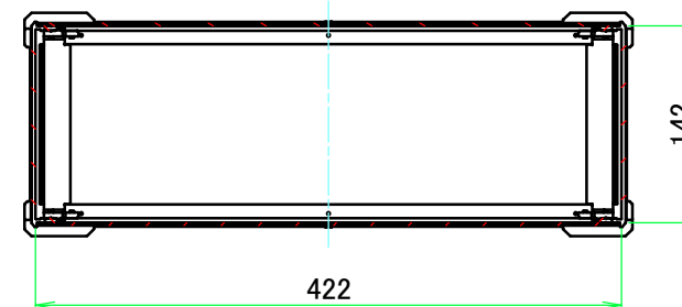
C-C (1:6)
