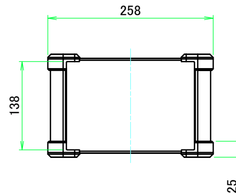
C view
