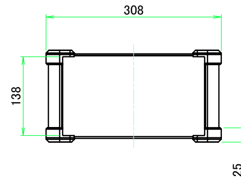
C view
