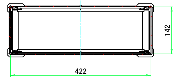
C-C (1:6.5)
