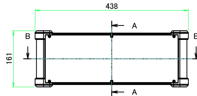
A view
